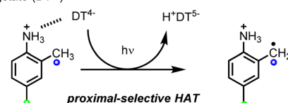
Scheme 14 Decatungstate-catalyzed site-selective C–H alkylation via electrostatic effects.
