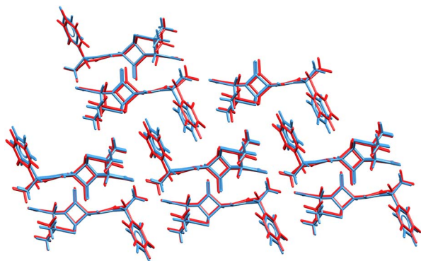
Fig. 12 Overlay of the ampicillin crystal structures determined from X-ray diffraction experiments 285 (blue) and the direct NMR crystallography solution (red) which employed a combination of DFTB energies and ShiftML chemical shifts. 261
