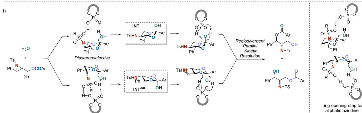
Scheme 3 Preliminary study of the mechanism: (a) reaction of substrate without assisting group. (b) Products interconversion experiment. (c) Isotopic labeling experiment. (d) Reactions with enantiopure substrate. (e) Steric effect studies. (f) Proposed mechanism.
