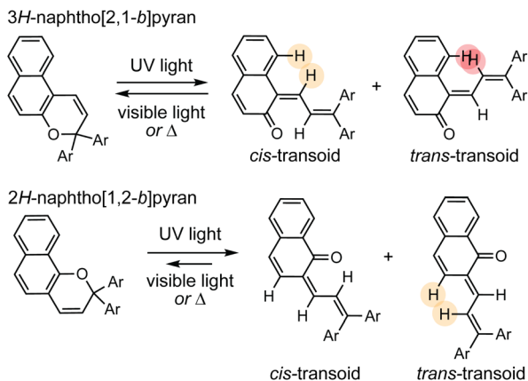
Scheme 11 The ring-opening reactions of 3H- and 2H-naphthopyrans generate merocyanine isomers with varying degrees of steric demand, which strongly influences absorption properties and reversion kinetics.
