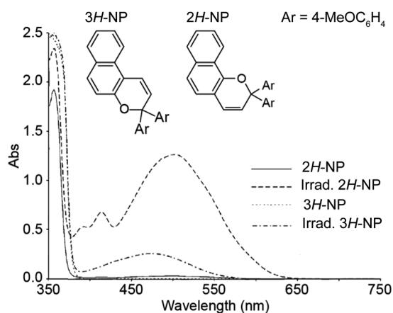
Fig. 4 UV-vis absorption spectra of 2,2-bis(4-methoxyphenyl)-2H-naphtho[1,2-b]pyran (2H-NP) and 3,3-bis(4-methoxyphenyl)-3H-naphtho[2,1-b]pyran (3H-NP) in toluene before and after irradiation with UV light. Adapted with permission from ref. 38. Copyright 2006, Elsevier.
