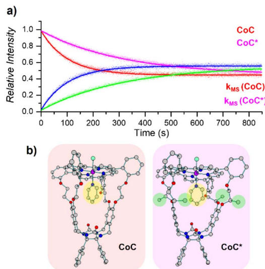
Fig. 6 (a) Relative time evolution of [\text{CoC}(\text{Py})_{\text{IN}}]^+ (red), [\text{CoC}(\text{Py}_{\text{I}})]^+ (blue), [\text{CoC}^*(\text{Py})_{\text{IN}}]^+ (magenta), and [\text{CoC}^*(\text{Py}_{\text{I}})]^+ (green) in a single DRL experiment carried out at 40 °C in \text{CHCl}_3 with 200 equiv. pyridine and 200 equiv. pyridine-D5. Dots are experimental data points, and lines correspond to fittings of experimental data by eqn (S1) and (S2). † (b) DFT-calculated structures of ^1[\text{CoC}(\text{Cl}_{\text{OUT}})(\text{Py}_{\text{IN}})] and ^1[\text{CoC}^*(\text{Cl}_{\text{OUT}})(\text{Py}_{\text{IN}})] optimized with B3LYP-D3/def2svp.
