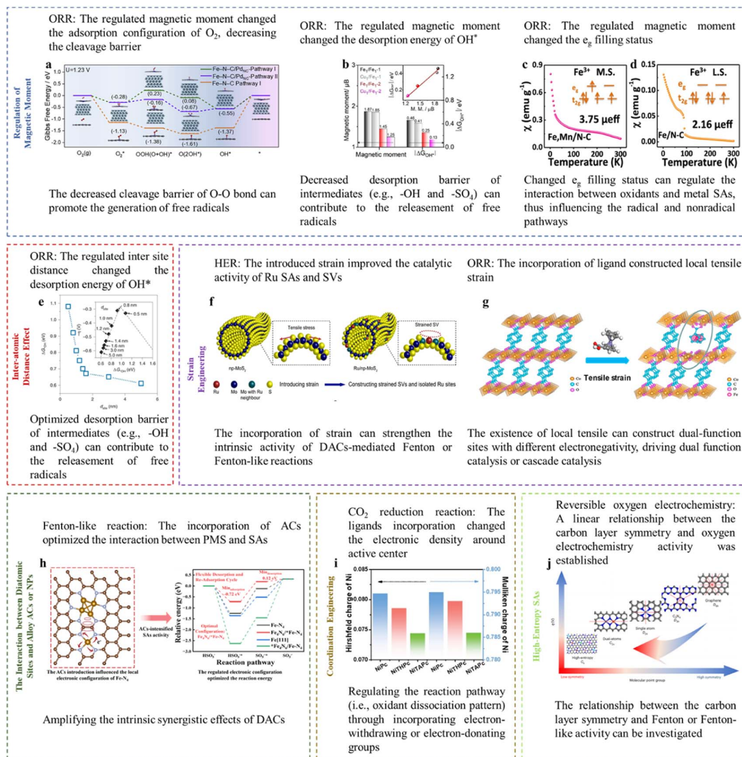
Fig. 3 (a) Gibbs free energy diagram of the ORR after the consideration of the solvent effect. Reprinted (adapted) with permission from ref. 16. Copyright 2022 Cell Press. (b) Comparison of the magnetic moment and \Delta G_{\text{O}^{\cdot\text{H}}^+} . Reprinted (adapted) with permission from ref. 17. Copyright 2022 Wiley. (c and d) Magnetic susceptibility of (c) Fe–Mn/NC, (d) Fe/NC (M. S. represents medium-spin, L. S. represents low-spin), with permission from ref. 18 copyright 2021 Springer Nature. (e) The d_{\text{site}} -dependent \Delta G_{\text{O}^{\cdot\text{H}}^+} obtained by DFT calculations. (Inset) Volcano plot of calculated overpotentials for the ORR against \Delta G_{\text{O}^{\cdot\text{H}}^+} . Reprinted (adapted) with permission from ref. 20. Copyright 2021 Springer Nature. (f) Illustration of the construction of Ru/np–MoS 2 . Reprinted (adapted) with permission from ref. 21. Copyright 2021 Springer Nature. (g) Crystal structures of CoBDC and CoBDC FcCA models obtained from DFT simulations. The microreactor is composed of directly coordinated carboxyl oxygen atoms of FcCA (Co1) and unsaturated coordinative Co2, together with the FcCA linker labeled by the circle. Reprinted (adapted) with permission from ref. 23. Copyright 2021 ACS. (h) The regulatory role of Fe ACs in the Fe SA-mediated PMS oxidation reaction. Reprinted (adapted) with permission from ref. 1. Copyright 2023 PNAS. (i) Hirshfeld and Mulliken charges of the Ni atom in NiPc, NiTHPc, and NiTAPc. Reprinted (adapted) with permission from ref. 30. Copyright 2021 Wiley. (j) The relationship between symmetry and electrocatalytic performance, with permission from ref. 32 copyright 2023 Springer Nature. Notably, high-resolution figures can be viewed in ESI (Fig. S4–S11†).
