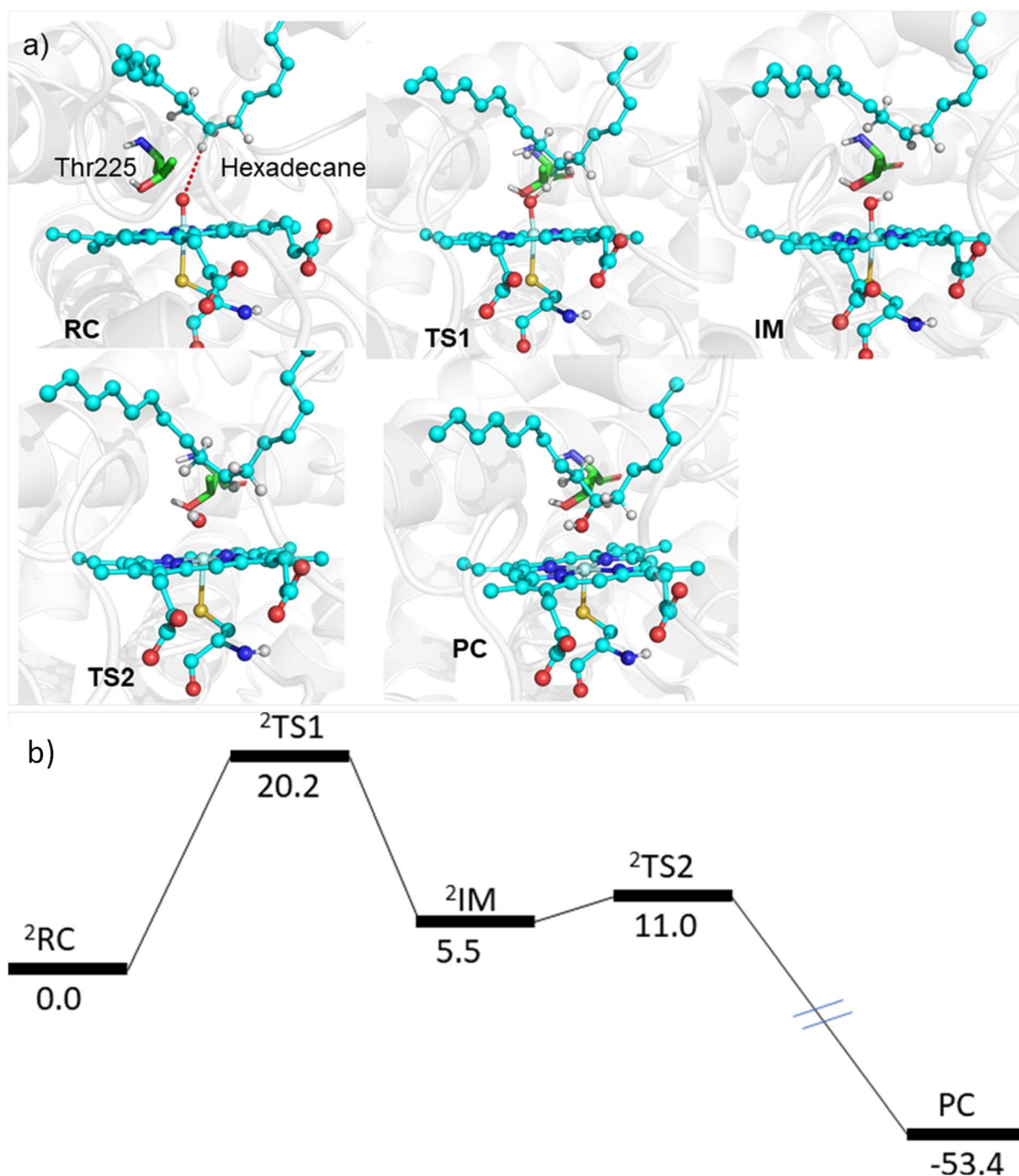
Fig. 5 (a) The geometry of different stationary points during the hydroxylation of hexadecane via compound I inside the active pocket of the LFFTFA mutant, (water molecules near the active site of the protein are not shown for the ease of representation). (b) The energy profile of the reaction obtained from QM/MM potential energy surface scanning using the UB3LYP-D3/def2-TZVP level of the theory. All energy values are in kcal mol -1 and the energy for PC is not scaled.
