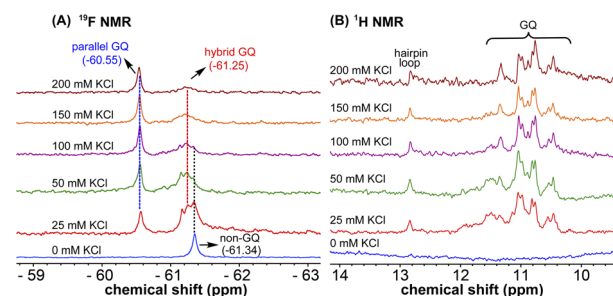
Fig. 6 (A) 19 F NMR and (B) 1 H NMR spectra of TFBF-modified ON 4 at different KCl concentrations.
