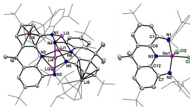
Fig. 2 Left: Solid-state structure of 2 . Right: solid-state structure of 3 . The t\text{-Bu} and Dipp groups are simplified as wireframes and hydrogen atoms are omitted for clarity. Thermal ellipsoids are set at the 30% probability level. Selected bond lengths (Å) and angles (°) for 2 : Li1–N1 1.890(4), Li1–N3 2.254(4), Li1–N5 1.903(4), Li1–N6 2.236(4), Li2–N2 2.013(5), Li2–N3 2.133(4), Li2–N5 1.992(4), Li3–N1 1.978(4), Li3–N4 2.000(4), Li3–N6 2.157(4), Li4–N2 2.030(4), Li4–N3 2.092(4), Li4–N4 2.038(4), Li4–N6 2.073(4). Selected bond lengths (Å) and angles (°) for 3 : Ge1–Cl1 2.091(2), Ge1–Cl2 2.163(2), Ge1–N1 2.011(2), Ge1–N2 2.039(2), Ge1–N3 1.872(2), C1–N1 1.387(3), C7–N2 1.379(3), C6–N3 1.349(3), C12–N3 1.362(3), C1–C6 1.404(3), C7–C12 1.402(3), N1–Ge1–N2 153.22(10), N1–Ge1–N3 80.34(8), N2–Ge1–N3 79.59(9), Cl1–Ge1–Cl2 104.09(10).
