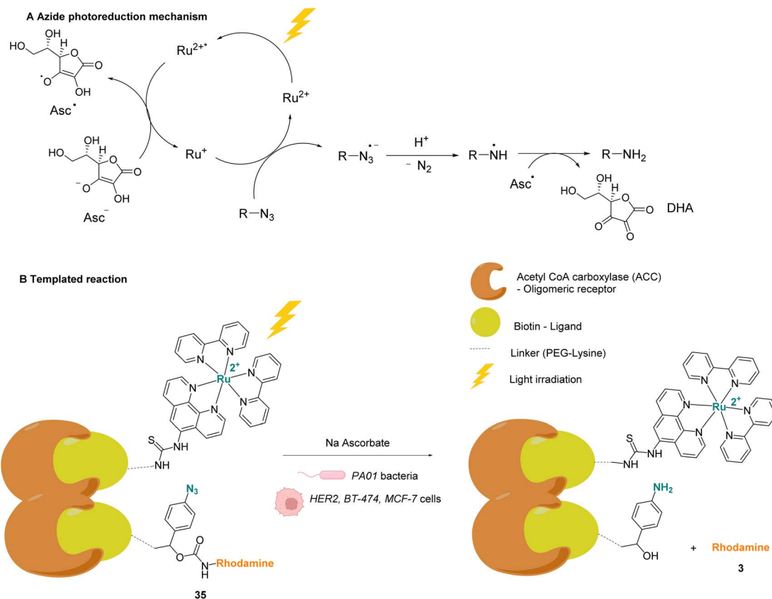
Fig. 12 (A) Mechanism of the photoreduction of the azide. (B) [Ru^{II}(bipy)_3] -type complexes and azide/rhodamine substrates linked to protein ligands for an intracellular protein templated reaction induced by visible light irradiation. Photoreduction of the azide to the aniline leads to immolative linker decomposition and uncaging of rhodamine. 47
