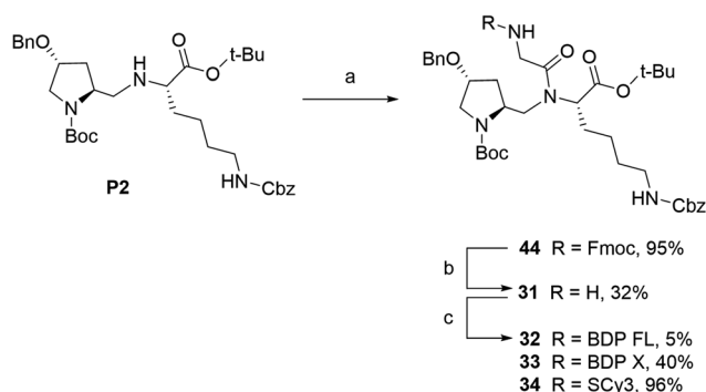
Scheme 1 Synthesis of fluorescent conjugates 32–34 . reagents and conditions: (a) dry DCM, N 2 , Fmoc-glycyl chloride 46 , 0 °C to rt, 30 min; (b) dry DMF, N 2 , diethylamine, rt, 1 h; (c) dry DMF ( 32 )/acetonitrile ( 33 , 34 ), N 2 , triethylamine, NHS-activated fluorophore, rt, 2 days ( 32 )/2 h ( 33 , 34 ).
