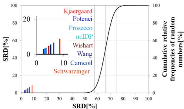
Fig. 8 SRD-CRRN results for C α SCS vectors of ubiquitin (BMRB 4769). Small-peptide RCCS predictors (Wishart, Schwarzsinger, Kjaergaard) are shown in shades of red, while database-derived ones (Wang, Camcoil, ncIDP, Prosecco, Potenci) are shown in shades of blue.
