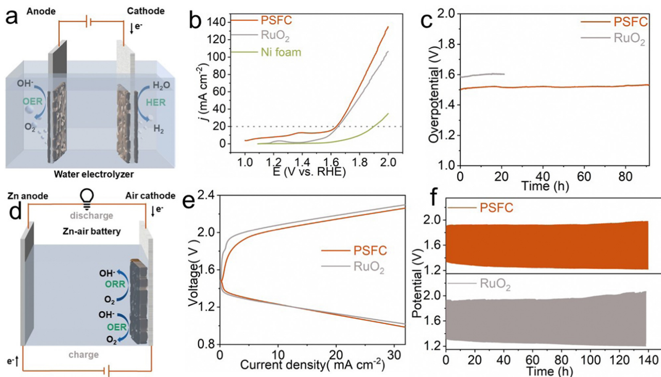
Fig. 5 (a) A schematic configuration of the water electrolyzer. (b) Polarization curves of bare Ni foam//Ni foam, Pt/C//PSFC, and Pt/C//RuO 2 (+) for overall water splitting in 0.1 M KOH at a scan rate of 5 mV s -1 . (c) Chronopotentiometry curve of water electrolysis using PSFC and RuO 2 as anodes respectively at a constant current density of 20 mA cm -2 in 0.1 M KOH. (d) A schematic configuration of Zn-air batteries. (e) Charge-discharge polarization curves of PSFC and Pt/C + RuO 2 based Zn-air batteries. (f) Long-term galvanostatic charge-discharge cycling profiles of ZABs with the Pt/C + RuO 2 electrocatalyst and PSFC electrocatalyst at 2 mA cm -2 .
