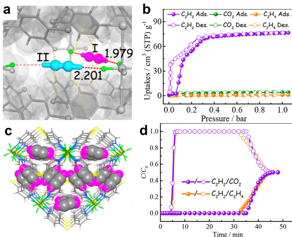
Fig. 9 (a) and (c) Neutron diffraction crystal structure of \text{UTSA-300-C}_2\text{H}_2 and (b) \text{C}_2\text{H}_2 , \text{CO}_2 , and \text{C}_2\text{H}_4 sorption isotherms for UTSA-300a at 273 K. (d) Experimental column breakthrough curves for equimolar \text{C}_2\text{H}_2/\text{CO}_2 (purple) and \text{C}_2\text{H}_2/\text{C}_2\text{H}_4 (orange) mixtures (298 K, 1 bar) in a fixed-bed packed with UTSA-300a. Reprinted with permission from ref. 72. Copyright 2017 American Chemical Society.
