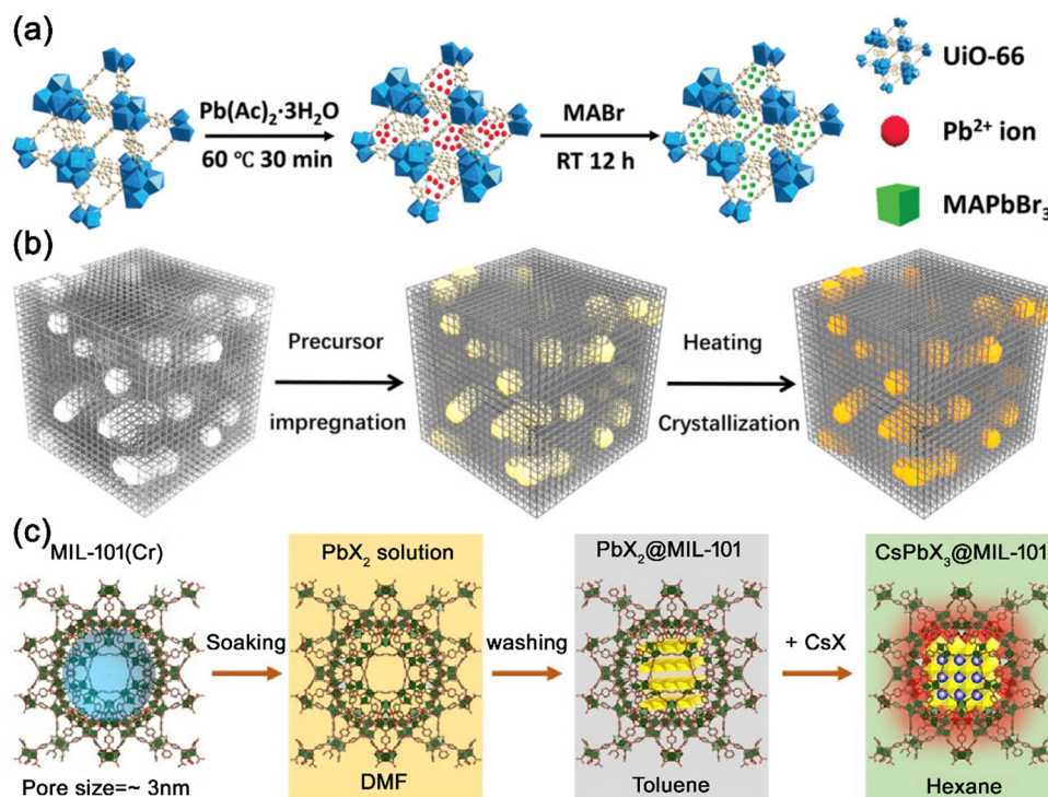
Fig. 13 (a) Schematic illustration of the in situ synthesis of \text{MAPbBr}_3 @UiO-66 composites through spontaneous formation. Adapted from ref. 130 with permission. Copyright 2020, Royal Society of Chemistry. (b) Schematic illustration of the in situ synthesis of \text{CsPbX}_3 @HP-UiO-66 composites triggered by changing the temperature. Adapted from ref. 131 with permission. Copyright 2021, Elsevier. (c) Schematic illustration of the in situ synthesis of \text{CsPbX}_3 @MIL-101 composites triggered by anti-solvents. Adapted from ref. 135 with permission. Copyright 2019, American Chemical Society.
