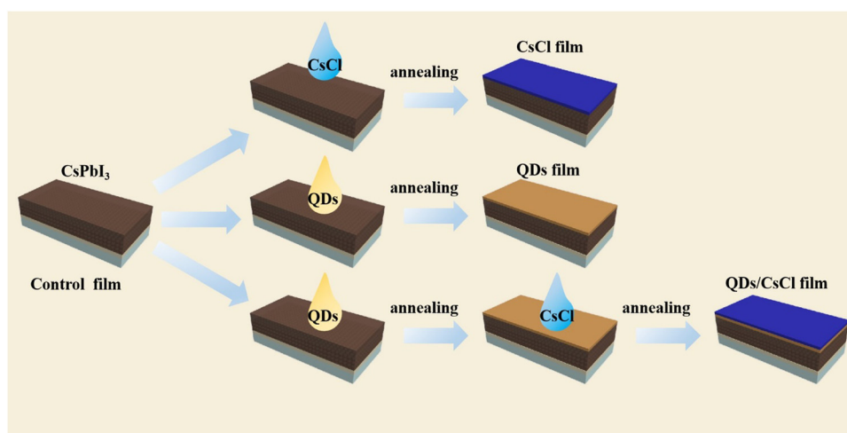
Fig. 1 Schematic illustrating the deposition processes of the \text{CsPbI}_3 - \text{CsCl} , \text{CsPbI}_3 -QDs and \text{CsPbI}_3 -QDs/ \text{CsCl} films.
