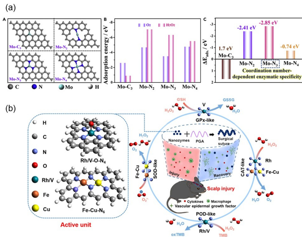
Fig. 8 (a) Construction of selective POD-like Mo SANs: (A) various potential POD-like models with optimized top structures; (B) adsorption energies for \text{O}_2 and \text{H}_2\text{O}_2 on \text{Mo-C}_3 , \text{Mo-N}_2 , \text{Mo-N}_3 , and \text{Mo-N}_4 structures; (C) differential values between \text{H}_2\text{O}_2 and \text{O}_2 adsorption energies on \text{Mo-C}_3 , \text{Mo-N}_2 , \text{Mo-N}_3 , and \text{Mo-N}_4 structures. Adapted with permission from ref. 117. Copyrights 2021, Elsevier. (b) Various active units result in differing activity levels within SANs, which find application in brain trauma healing through the promotion of vascular endothelial growth factor expression and the reduction of oxidative stress and inflammation. Adapted with permission from ref. 118. Copyright 2022, the authors.
