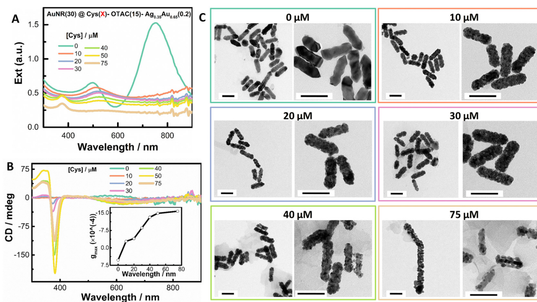
Fig. 2 Effect of Cys concentration on the formation of island helical shells mediated by OTAC (15 mM). (A) Extinction and (B) CD spectra. Inset: g_{max} vs. Cys concentration. (C) Typical TEM images of AuNR(30)@Cys(X)-OTAC(15)-Ag 0.35 Au 0.65 (0.2) nanostructures obtained at different Cys concentrations. Scale bar: 100 nm.
