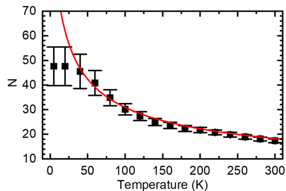
Fig. 7 Average number of thiophene rings N in a conjugated segment that gives rise to PL emission at a given temperature, calculated from eqn (4) using the data in Fig. 4(a). The red line denotes the values based on the extrapolation to 0 K (dashed line in Fig. 4(a)), the black squares are based on the experimental data (black squares in Fig. 4(a)).
