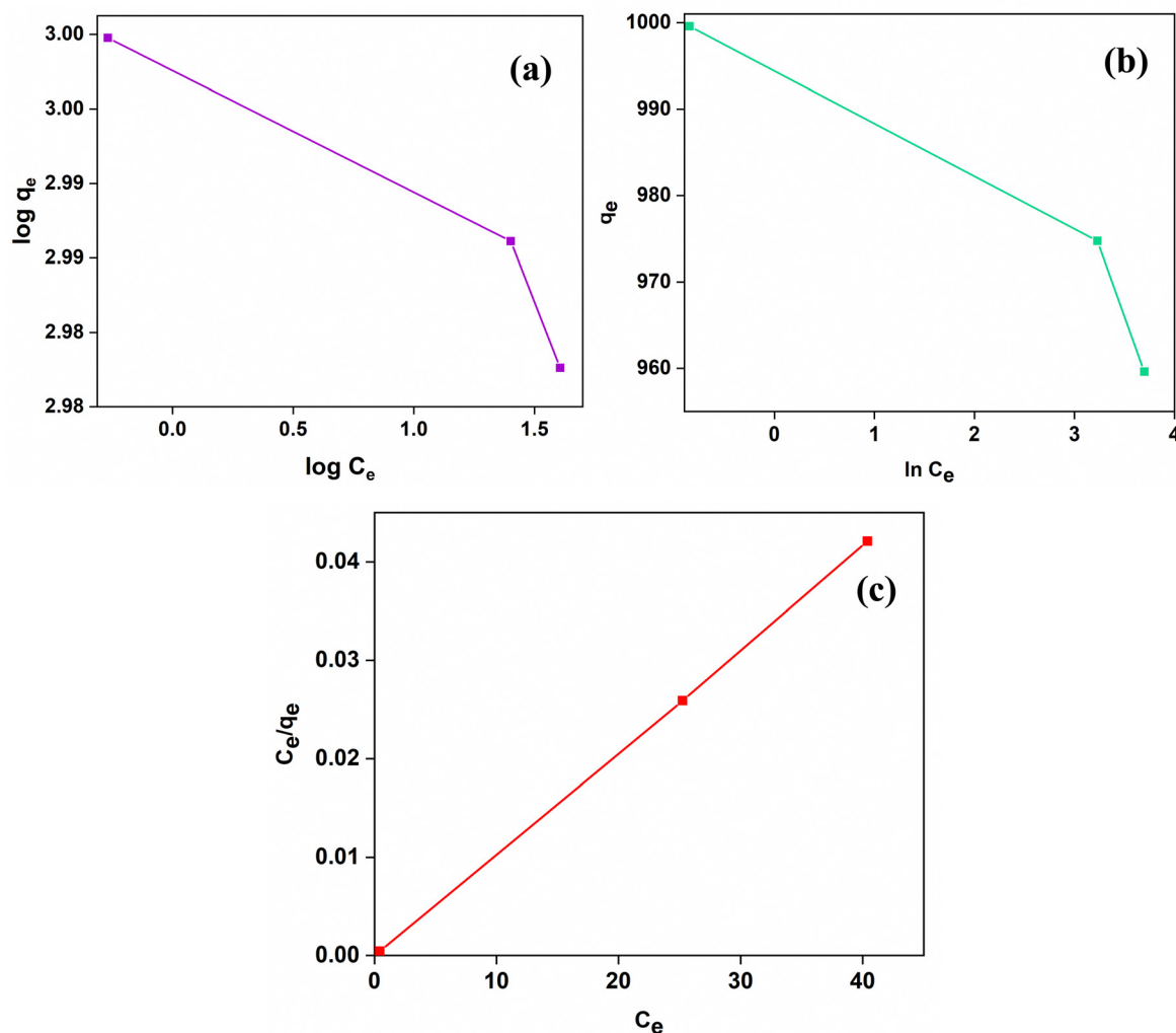
Fig. 9 Adsorption isotherms for 5 \mu\text{M} CR adsorption by SnO 2 at pH = 5 and room temperature. (a) Freundlich isotherm, (b) Temkin isotherm and (c) Langmuir isotherm.
