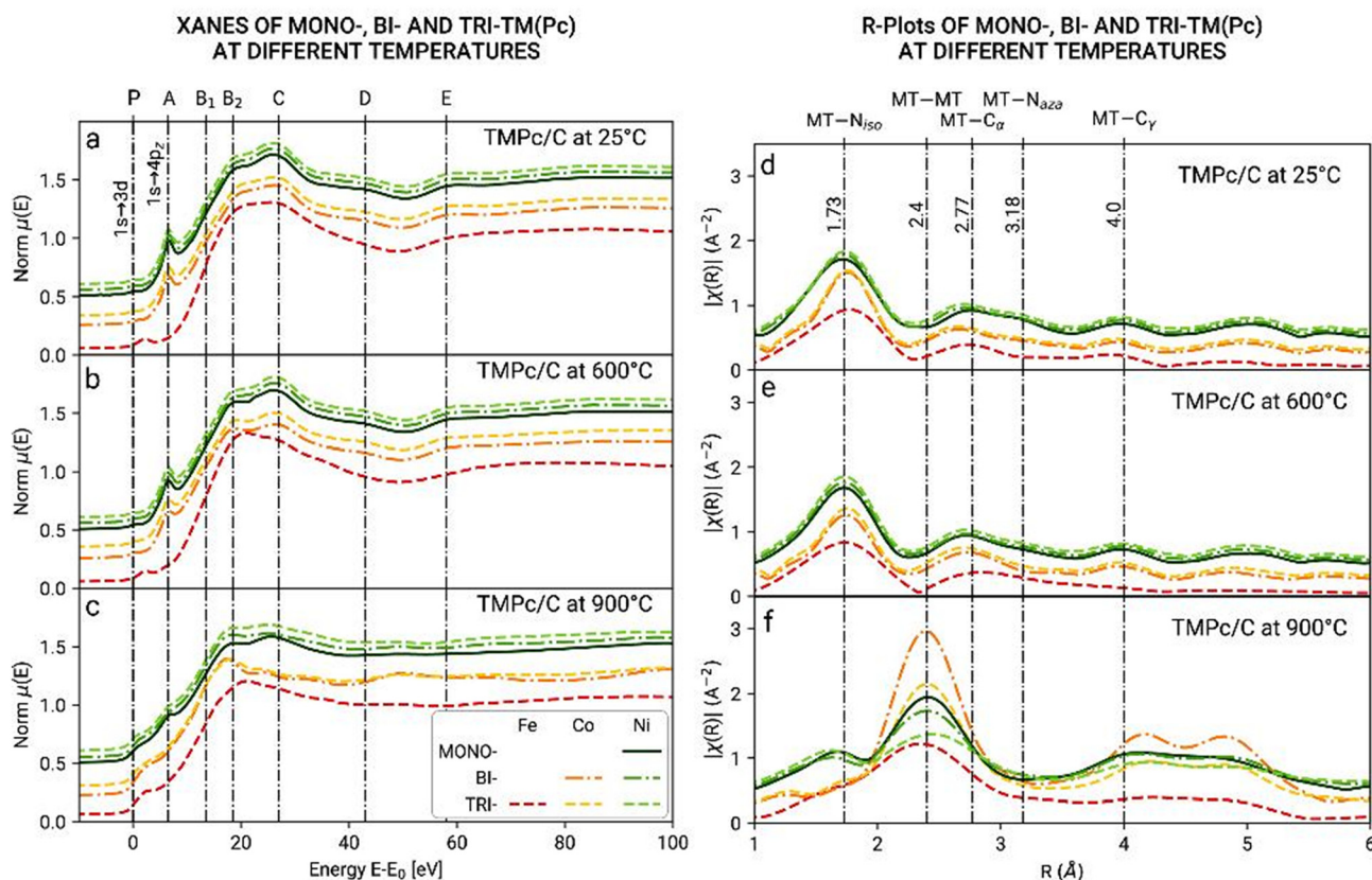
Fig. 8 Plots on the left (a–c): normalized XANES spectra of the transition metals in the range E-E_0 \in [-10-100] eV, where E_0 is the K edge. The spectra are grouped by element, each one with a corresponding color: green for Ni, yellow for Co, and red for Fe. The shape of the line is representative of the sample: solid for the Ni monometallic, dot-dash for the Ni-Co bimetallic sample, and dashed line for the Ni-Fe-Co trimetallic electrocatalysts. (a) The spectra collected on the samples at room temperature. (b) The ones collected after heating the samples at 600 °C. (c) The spectra collected after pyrolysis at 900 °C. Plots on the right (d–f): FT EXAFS-plots ( R ) of the transition metals, phase-corrected; (d) spectra collected at room temperature; (e) after heating treatment at 600 °C; and (f) after pyrolysis at 900 °C.
