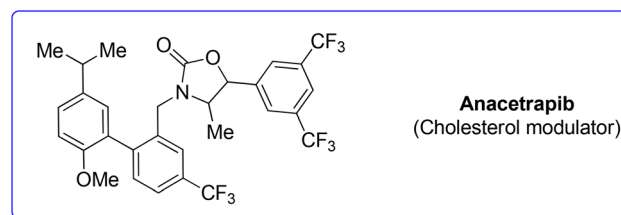
Scheme 6 Anacetrapib chemical structure.
