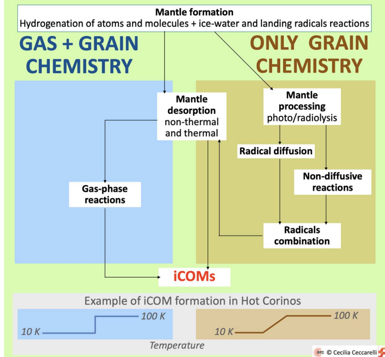
Fig. 9 Sketch of the two major scenarios invoked in the literature for the formation of iCOMs: "Gas + grain chemistry" and "Only grain chemistry". Both predict the formation of icy mantles enveloping the interstellar dust grains, prevalently during the cold molecular cloud and prestellar core stages. The mantle constituents are the result of the hydrogenation of atoms and simple molecules, such as CO, and the oxidation. Water and methanol, for example, are formed in this first step. 121–123 In addition, after the first layers of water-ice are formed, radicals landing on the grain surfaces can react with the ice-water molecules. The iCOM ethanol, for example, can be formed in this way. 124 After this first step, the two scenarios differ as follows. Left blue panel: In the "Gas + grain chemistry" scenario, the mantle components are either partially or completely injected into the gas-phase by thermal and non-thermal desorption processes, where they undergo gas-phase reactions that form iCOMs. This can occur either via mantle thermal desorption in hot corinos and inner protoplanetary disks, or via mantle non-thermal desorption in prestellar cores, outer protoplanetary disks and molecular outflows. Right brown panel: In the "Only grain chemistry" scenario, the icy mantles are processed by UV (photolysis) and CR (radiolysis) irradiation while being formed, and the radicals formed by the two processes remain trapped in the ice. When the dust temperature increases, radicals on the mantles become mobile and diffuse and, when they meet or meet some closed-shell species, they combine forming iCOMs. Alternatively, non-diffusive processes can also combine radicals into iCOMs. Likewise, some radicals are also predicted to meet and react in non-diffusive processes during the cold phase.
