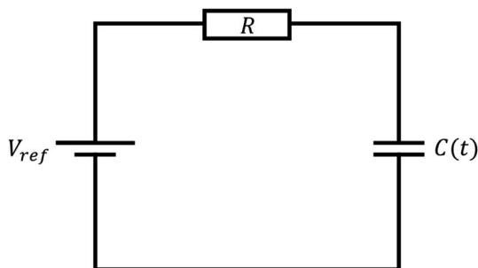
Fig. 1 Schematic of the electrical circuit and the principle of the reverse capacitive actuation. A time-varying capacitor C(t) is connected in series to a low-voltage battery, V_{ref} and an electric load, R . Varying the capacitance periodically, by using mechanical work, creates alternating current of electrons through the circuit.
