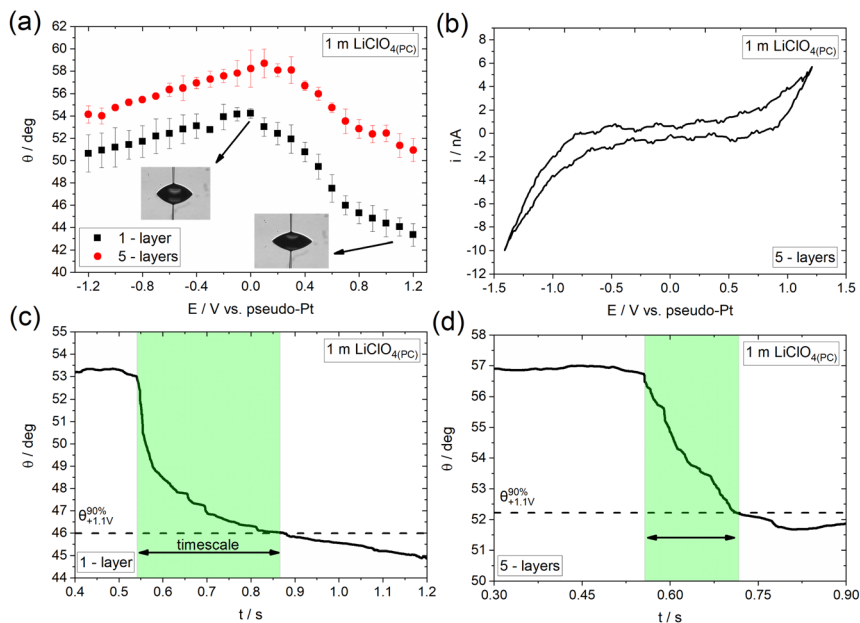
Fig. 5 (a) Change in apparent equilibrium electrostatic contact angle, \theta , with the applied bias (values are reported vs. Pt wire pseudo-reference electrode) at the CVD graphene|1 m LiClO 4 (PCl) interface for 1- and 5-layers thickness. Measurements were conducted under static conditions based on the protocol described in the Experimental section. (b) Cyclic voltammogram recorded at a 1 m LiClO 4 (PCl) droplet on 5-layers graphene using a scan rate of 100 mV s -1 . Timescales (highlighted regions) during a wetting cycle in 1 m LiClO 4 (PCl) following the protocol described in the Experimental section for (c) 1- and (d) 5-layers CVD graphene. The depicted cycle corresponds to a potential pulse from 0 V to +1.1 V vs. pseudo-Pt, i.e. , in the potential region where ClO 4 - anion adsorption/intercalation occurs.
