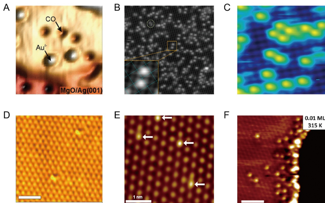
Fig. 2 (A) STM image of Au atoms and CO molecules on the MgO surface. Reproduced with permission. 5 Copyright © 2010, American Chemical Society. (B) Atomic-resolution STM image of Au-deposited Fe 3 O 4 (001). Reproduced with permission. 6 Copyright © 2012 American Physical Society. (C) STM image acquired after deposition of 0.2 monolayer Pd on the Fe 3 O 4 (001) surface at room temperature. Reproduced with permission. 7 Copyright © 2013, Springer Nature Limited. (D) High-resolution STM image of a region above a step edge where individual Pd surface atoms reside. Reproduced with permission. 8 Copyright © 2012, American Association for the Advancement of Science. (E) Isolated Pd atoms (highlighted by arrows) substituted into the Au(111) surface that appear slightly topographically higher than the Au host. Reproduced with permission. 9 Copyright © 2016, American Chemical Society. (F) Atomic resolution STM image revealing Pt alloys in the surface at the ascending step edges. Reproduced with permission. 10 Copyright © 2014, American Chemical Society.
