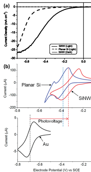
Fig. 9 (a) PEC HER performance comparison of the Si nanowire and planar Si. (b) Cyclic voltammograms of methylviologen on the Si nanowire and planar Si photoelectrode under illumination and on the Au electrode in the dark. Reproduced with permission from ref. 81, Copyright © 2012, American Chemical Society.
