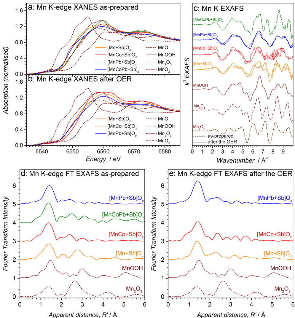
Fig. 2 Mn K-edge (a and b) XANES, (c) EXAFS and (d and e) FT EXAFS data collected for the [Mn + Sb]O x (orange), [MnCo + Sb]O x (red), [MnPb + Sb]O x (blue) and [MnCoPb + Sb]O x (green) catalysts before and after OER tests (10 mA cm -2 , 24 h, 24 ± 2 °C) compared to relevant reference materials (see figure). In panel c, dashed and solid traces show data collected before and after the OER tests, respectively.
