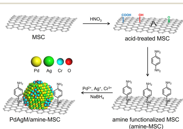
Scheme 1 Schematic illustration of the synthesis of the PdAgCr-supported amine-MSC catalyst.
