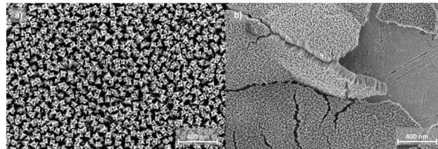
Fig. 1 SEM images of a 120 nm NiO thin film on Au a) before and b) after electrochemistry.
