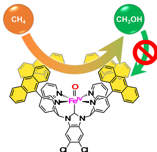
Fig. 7 The concept of "catch and release" strategy to suppress the overoxidation for selective conversion of methane to methanol. 62
