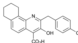
35 PSI-697 \text{IC}_{50} = 125 \mu\text{M} (P-selectin)
