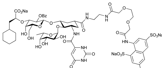
31 GMI-1070/Rivipansel \text{IC}_{50} = 4.3 \mu\text{M}
