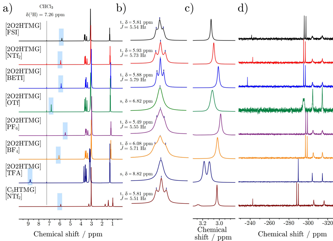
Fig. 4 (a) ^1\text{H} -NMR spectra of the pure ionic liquids using external \text{CDCl}_3 as reference. (b) Zoom on the shape of the acidic proton with chemical shift and coupling constant. For the samples with the [\text{OTf}]^- and [\text{TFA}]^- anion singlets are observed, while for all other anions triplets are found. (c) Signals of the \text{N}(\text{CH}_3)_2 groups. The [\text{2O2HTMG}][\text{TFA}] shows two singlets for the \text{N}(\text{CH}_3)_2 protons which indicates rotamers ( k_{\text{rot}} \ll \Delta\nu ). (d) ^{15}\text{N} -NMR spectra of the protic ionic liquids. For all samples, besides the [\text{OTf}]^- and [\text{TFA}]^- ionic liquid, the signal of the protonated N (located at -298 to -288 ppm) is a doublet, showing a coupling with the acidic proton. Signals located at approximately -315 ppm and -305 ppm result from the two \text{N}(\text{CH}_3)_2 groups, and those at -240 ppm and result from the imide nitrogen of the anions. All spectra are recorded at T = 298 K.
