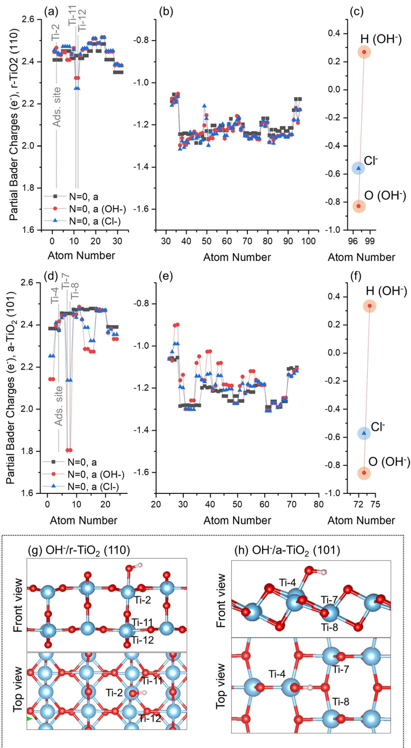
Fig. 4 Partial Bader charges for ground state (singlet, N = 0 ) electronic structure of clean, hydroxyl-, and chloride-containing (a–c) r - \text{TiO}_2 (110) and (d–f) a - \text{TiO}_2 (101) surfaces. Charges over Ti ions (a and d), O ions (b and e), and adsorbates (c and f) are individually presented. Inserts show representative example of adsorbate-containing surface (g: OH ^- /r-TiO _2 (110); h: OH ^- /a-TiO _2 (101)). Atom numbers refer to labels defined in the methodology section.
