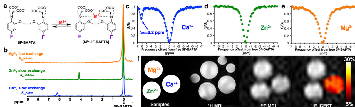
Fig. 6 The iCEST approach. (a) The dynamic exchange process between free 5F-BAPTA and M^{2+} -bound [M^{2+}\text{-5F-BAPTA}] . (b) ^{19}\text{F} NMR spectra of 5F-BAPTA in the presence of \text{Mg}^{2+} , \text{Zn}^{2+} , or \text{Ca}^{2+} . (c–e) Shown are ^{19}\text{F} -iCEST Z-spectra of solutions containing 10 mM 5F-BAPTA and 50 \mu\text{M} M^{2+} . (f) ^1\text{H} -MRI, ^{19}\text{F} -MRI, and iCEST ( \Delta\omega = 6.2 ) of M^{2+} solutions. Reproduced with permission from ref. 73.
