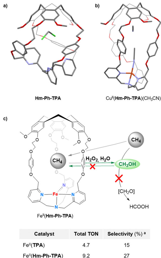
Fig. 9 Representation of the XRD structures of (a) Hm-Ph-TPA and (b) Cu II (Hm-Ph-TPA) . (c) Concept of the selective methane to methanol oxidation via H 2 O 2 activation in Fe II (Hm-Ph-TPA) , in water along with the comparison table between the open Fe II (TPA) and the caged catalysts. a Selectivity toward primary oxidation products CH 3 OH and CH 3 OOH.
