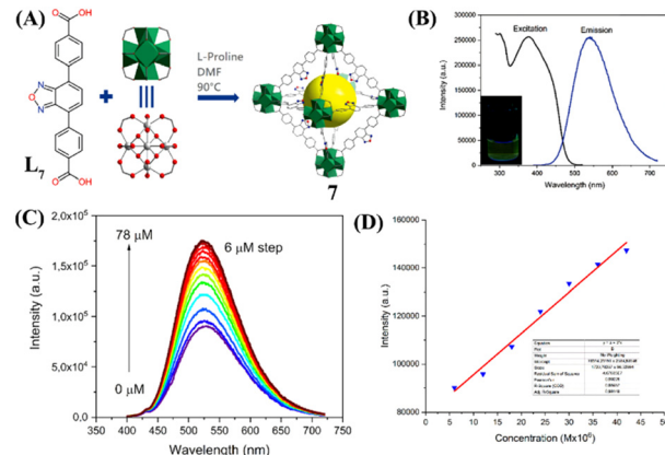
Fig. 4 (A) Synthesis of sensor LMOF 7 from ligand L_7 and Zr(IV); (B) Excitation and emission spectra of 7 were measured in \text{H}_2\text{O} (inset: photographs of 7 in \text{H}_2\text{O} ); (C) Changes in fluorescence emission intensity for 7 upon the gradual addition of aqueous \text{NH}_3 . (D) Linear fit for the \text{NH}_3 concentration–intensity correlation. Reprinted with permission from ref. 51. Copyright 2022 Royal Society of Chemistry.
