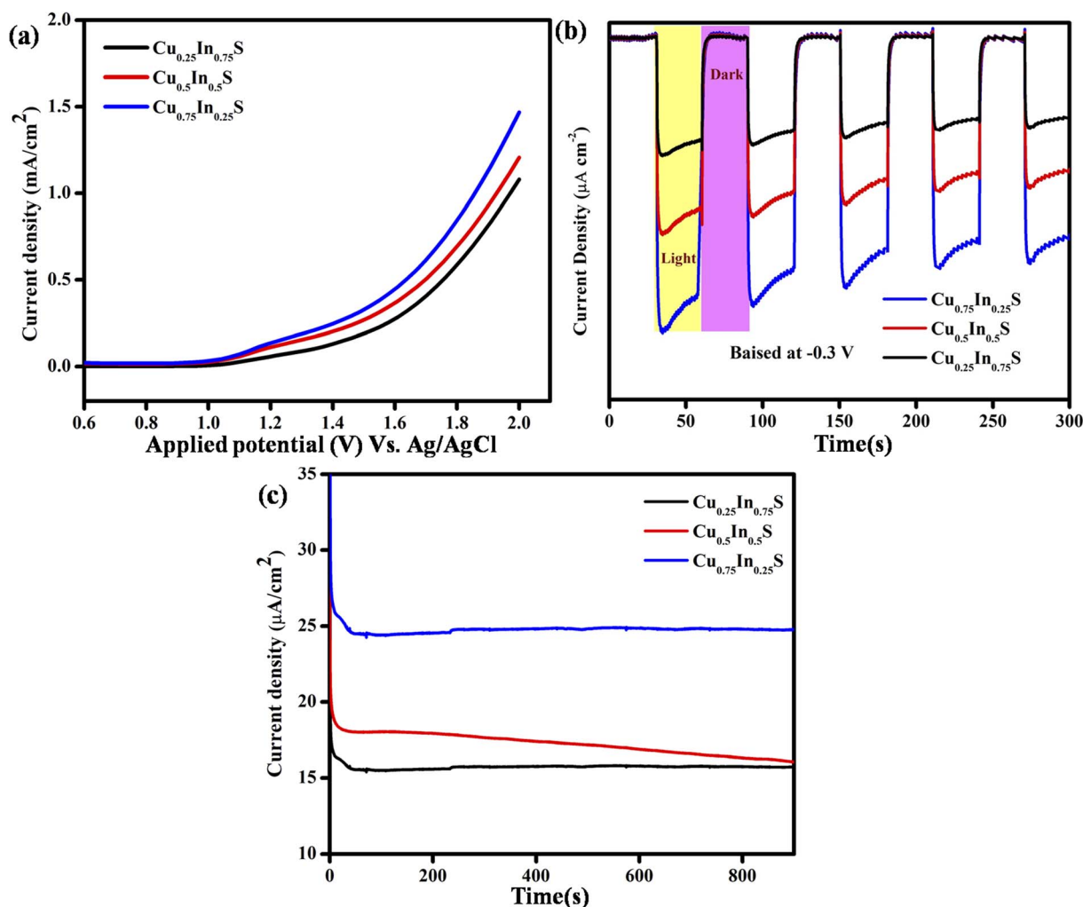
Fig. 3 Photocurrent study of the synthesized materials with various Cu/In ratios: (a) LSV plot, (b) TPC response at -0.3 \text{ V} biasing potential, and (c) CA plot at 0.2 \text{ V} applied potential.
