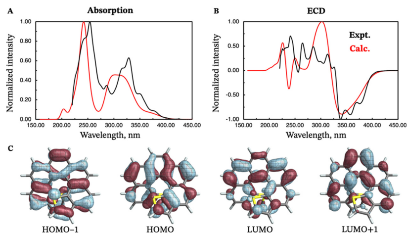
Fig. 8 Experimental (black curves) and calculated (red curves) absorption (panel A) and ECD (panel B) spectra of (M) -endo-dithia[7]helicene 11 . Isosurfaces ( \pm 0.03 au) for the most relevant frontier molecular orbitals (HOMO-1, HOMO, LUMO, and LUMO+1) are shown in panel C. The calculated energies were shifted by -0.40 eV prior to conversion to wavelengths.
