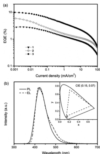
Fig. 10 (a) The EQE–current density characteristics of the OLEDs based on (1) DPA-DPS , (2) TDPA-DPS and (3) TDTC-DPS . (b) The EL and PL spectra of 10 wt% TDTC-DPS doped in a DPEPO layer. Inset: The CIE coordinates of the EL spectrum of a TDTC-DPS -based device. Reproduced with permission from ref. 53. Copyright 2012 American Chemical Society.
