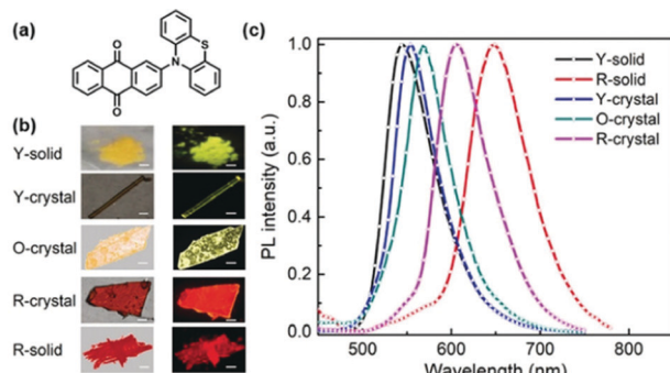
Fig. 34 (a) The molecular structure of PTZ-AQ . (b) Photographs of the five solid states of PTZ-AQ (left: under ambient light; right: under UV excitation; scale bar: 200 mm). (c) PL spectra of PTZ-AQ in different aggregation states. Reproduced with permission from ref. 96. Copyright 2018 John Wiley & Sons.
