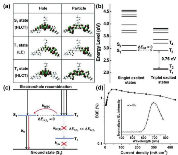
Fig. 25 (a) Natural transition orbitals for S_1 , T_1 , and T_3 states of PTZ-BZP . (b) The energy landscape for singlet and triplet excited states. (c) Model for exciton relaxation in the EL process. RISC: reverse intersystem crossing; IC(T): internal conversion between the triplet states; fl: fluorescence; ph: phosphorescence. (d) EQE-current-density characteristics of the device. The inset graph shows the EL spectrum. Reproduced with permission from ref. 36. Copyright 2014 John Wiley & Sons.
