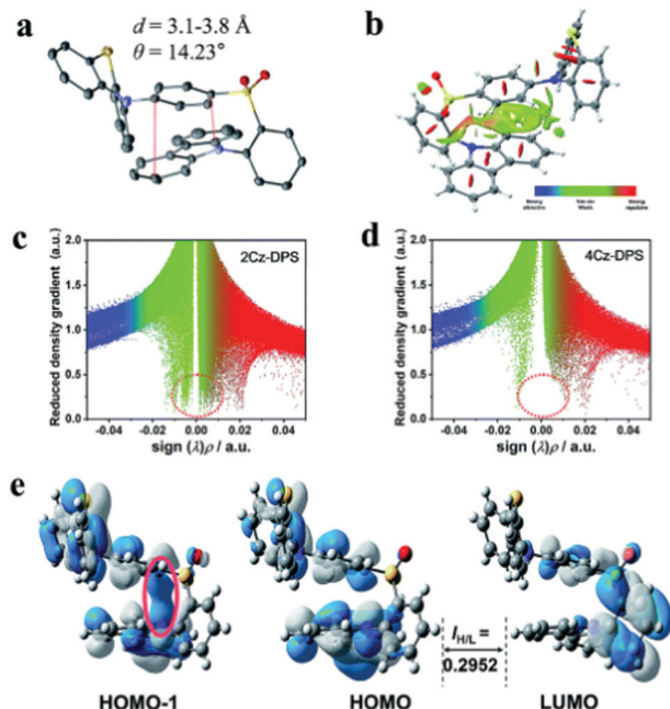
Fig. 15 (a) Single crystal and (b) reduced density gradient (RDG) isosurface map with an isovalue of 0.5 for 2Cz-DPS . (c and d) The functions of RDG and \text{Sign}(\lambda_2)\rho for 2Cz-DPS and 4Cz-DPS , respectively. (e) HOMO and LUMO distribution of 2Cz-DPS , showing the overlapping integral extents I_{H/L} .
