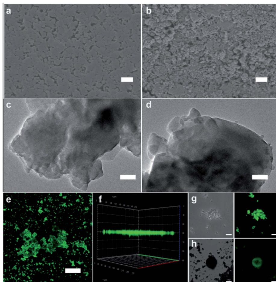
Fig. 3 Characterization of GOx/ZIF-8-WV. 54 (a) SEM image of pressed GOx/ZIF-8 (scale bar: 1\ \mu\text{m} ). (b) SEM image of GOx/ZIF-8-WV (scale bar: 1\ \mu\text{m} ). (c) TEM image of pressed GOx/ZIF-8 (scale bar: 100\ \text{nm} ). (d) TEM image of GOx/ZIF-8-WV (scale bar: 100\ \text{nm} ). (e) Laser confocal fluorescence microscopy imaging of the FITC-GOx/ZIF-8-WV (scale bar: 50\ \mu\text{m} ). (f) 3D reconstruction of laser confocal fluorescence microscopy imaging of the FITC-GOx/ZIF-8-WV. (g) Laser confocal fluorescence microscopy imaging of the FITC-GOx/ZIF-8-WV (scale bar: 5\ \mu\text{m} ). (h) Laser confocal fluorescence microscopy imaging of the FITC-GOx-on-ZIF-8 (scale bar: 10\ \mu\text{m} ).
