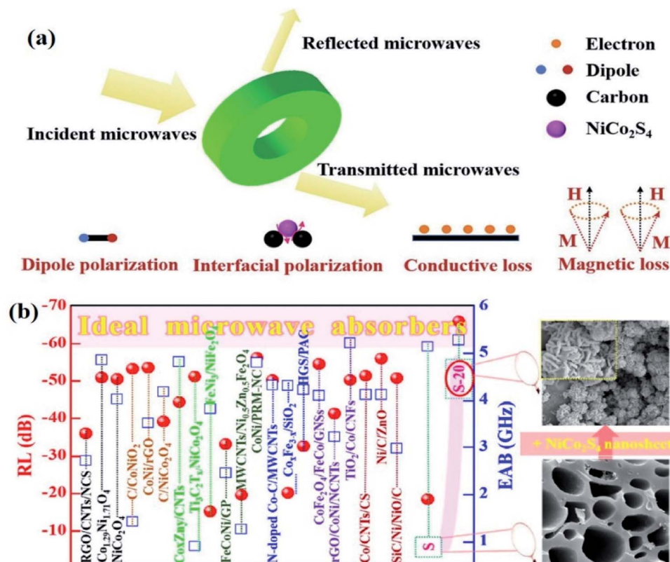
Fig. 14 Proposed microwave absorption mechanism of NCS-based materials (a) and comparison of microwave absorption ability among different materials (b). 163 Reproduced from ref. 121 with permission from Elsevier.
