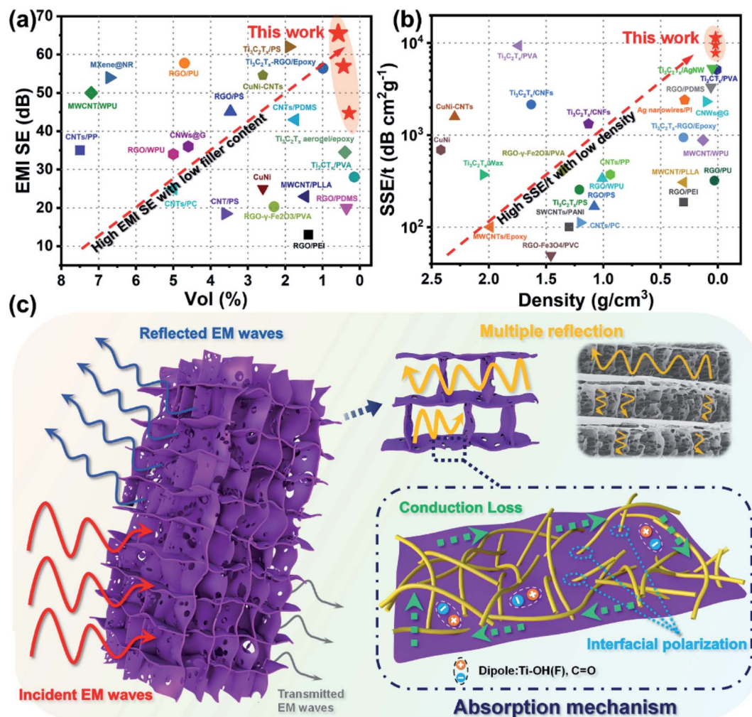
Fig. 6 (a) EMI SE versus \text{Ti}_3\text{C}_2\text{T}_x content (vol%) and (b) \text{SSE}/t versus density of the anisotropic \text{Ti}_3\text{C}_2\text{T}_x/\text{ANF} aerogels compared with previous reports. (c) Electromagnetic shielding mechanism of the anisotropic \text{Ti}_3\text{C}_2\text{T}_x/\text{ANF} aerogel.
