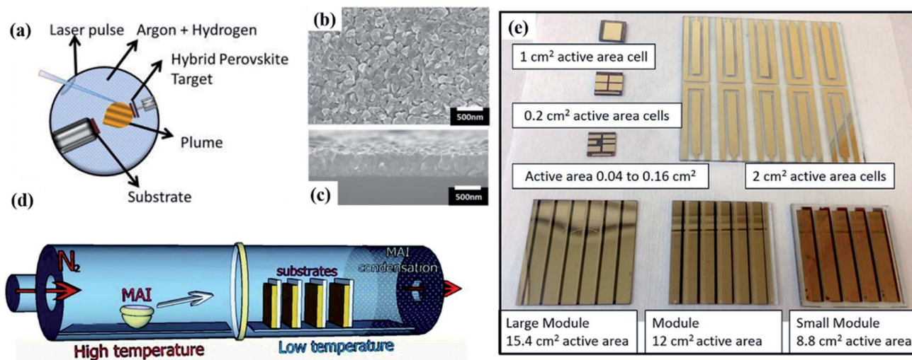
Fig. 4 (a) Schematic diagram of the PLD configuration and deposition process 103 (b) top view of PVK film on silicon wafer deposited with PLD 103 (c) the cross-section of the PLD PVK film 103 (d) schematic diagram of the HCVD configuration for MAI deposition onto PbI 2 coated substrates 109 (e) image of cells and modules prepared with HCVD approach demonstrating the up-scaling process. 110
