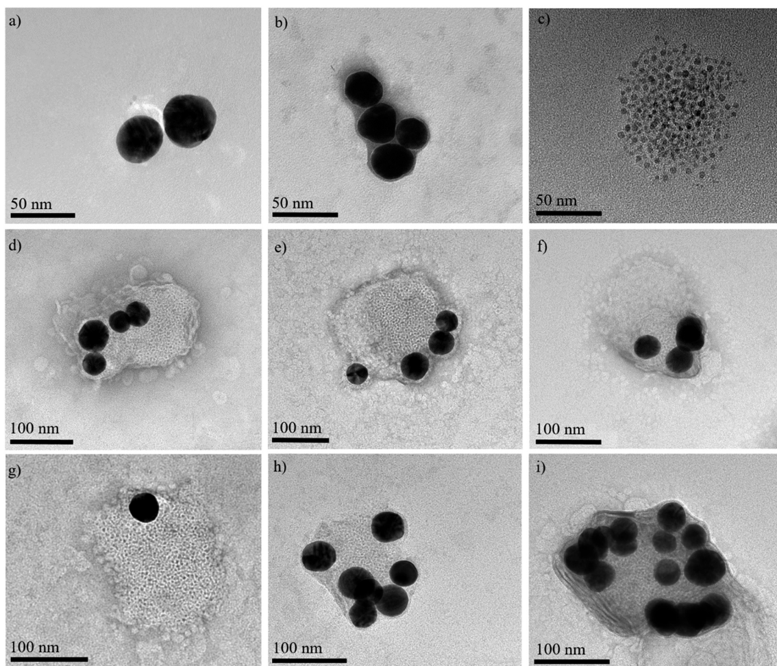
Fig. 5 Representative TEM images of a) TNB-functionalized AuNPs, b) AuNP-loaded niosomes, c) Fe 3 O 4 NPs/NIO, d)–i) AuNPs/Fe 3 O 4 NPs/NIO hybrid niosomes.
