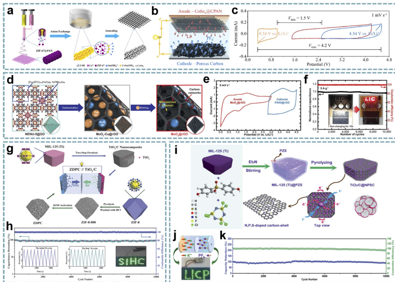
Fig. 10 MOF-derived metal/carbons for MIHCs. (a) Schematic diagram of the fabrication process of CoSn x @CPAN nanofibers. (b) Schematic of the configuration of a full-cell LIHC. (c) CV profiles from a three-electrode device. Reproduced with permission from ref. 189. Copyright 2020, Elsevier. (d) Schematic diagram of the fabrication process of the MoO 2 @rGO anode. (e) CV curves of the MoO 2 @rGO anode and PANI@rGO cathode at a scan rate of 5 mV s -1 . (f) Charge–discharge cycling stability at 5 A g -1 with a wireless charging kit charged by a solar cell. Reproduced with permission from ref. 78. Copyright 2020, Wiley-VCH. (g) Construction process of the TiO 2 /C anode and ZDPC cathode. (h) Cycling performance and coulombic efficiency of the TiO 2 /C//ZDPC SIHC under 1 A g -1 . Reproduced with permission from ref. 193. Copyright 2018, Wiley-VCH. (i) Schematic diagram of the preparation process of TiO 2 /C@NPSC. (j) LED arrays powered by the PIHC device. (k) Cycling performance and coulombic efficiency. Reproduced with permission from ref. 80. Copyright 2020, Royal Society of Chemistry.
