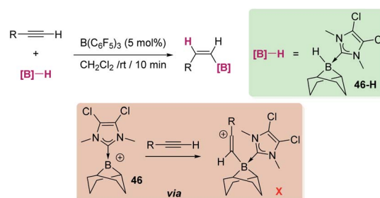
Scheme 54 Hydroboration of alkynes catalysed by \text{B}(\text{C}_6\text{F}_5)_3 .
