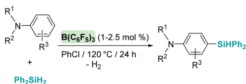
Scheme 51 CH silylation of anilines catalysed by \text{B}(\text{C}_6\text{F}_5)_3 .
