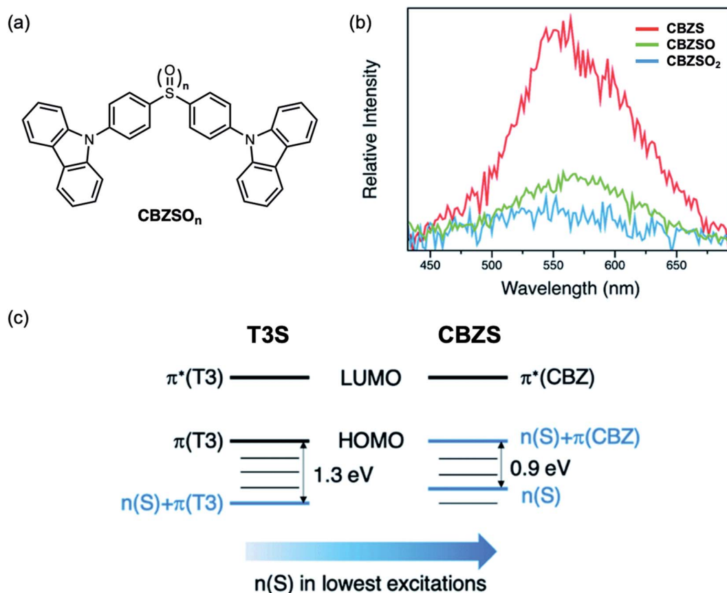
Fig. 11 (a) Structures of sulfur-bridged carbazole dimers CBZSO n reported by our group. (b) Time-resolved photoluminescence spectra (60 μs to 110 ms time range) of CBZS, CBZSO and CBZSO 2 crystalline samples under ambient conditions at 298 K. The intensity is corrected by fluorescence integration under the same excitation condition as time-resolved measurements and PLQYs. (c) Schematic comparison of frontier orbitals in terthiophene (T 3 S) and carbazole (CBZS) sulfur-bridged dimers. Adapted with permission from ref. 59. Copyright 2021 Royal Society of Chemistry.
