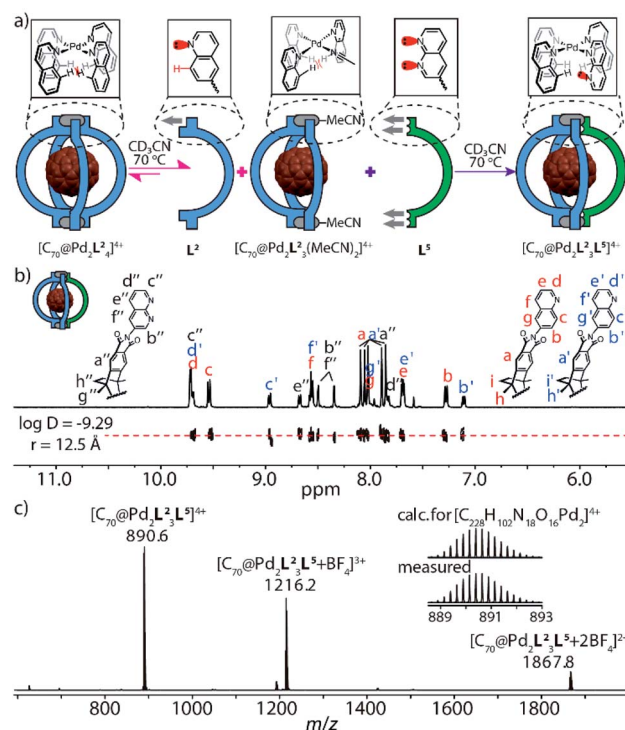
Fig. 3 Self-assembly and characterization of heteroleptic cage [C_{70}@Pd_2L_3L^5] : (a) when bowl [C_{70}@Pd_2L_3(MeCN)_2] reacts with ligand L^2 or L^5 in a 1 : 1 ratio at 70^\circ C , the former ligand only yields minor amounts of cage [Pd_2L_4] while the latter leads to quantitative conversion; (b) ^1H NMR and DOSY spectra (600 MHz, 298 K, CD_3CN ) of cage [C_{70}@Pd_2L_3L^5] (0.64 mM); (c) high-resolution ESI mass spectrum of [C_{70}@Pd_2L_3L^5] and BF_4^- adducts.
