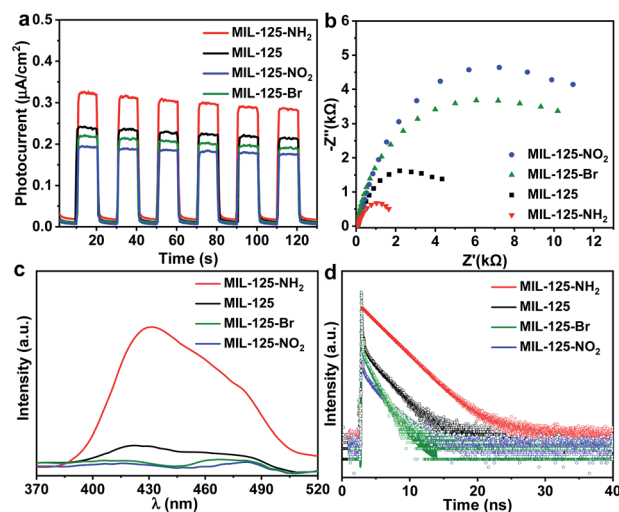
Fig. 3 (a) Photocurrent responses, (b) EIS Nyquist plots, (c) photoluminescence (PL) spectra (excited at 250 nm), and (d) time resolved PL spectra for MIL-125 and MIL-125-X ( X = \text{NH}_2 , \text{NO}_2 , \text{Br} ) in MeCN.
